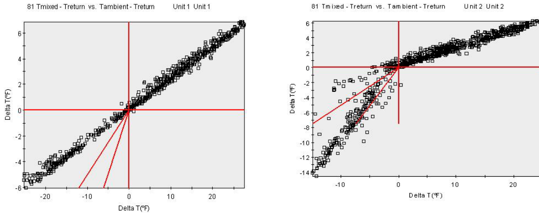
Figure 7.11: Economizer Diagnostic Plots
