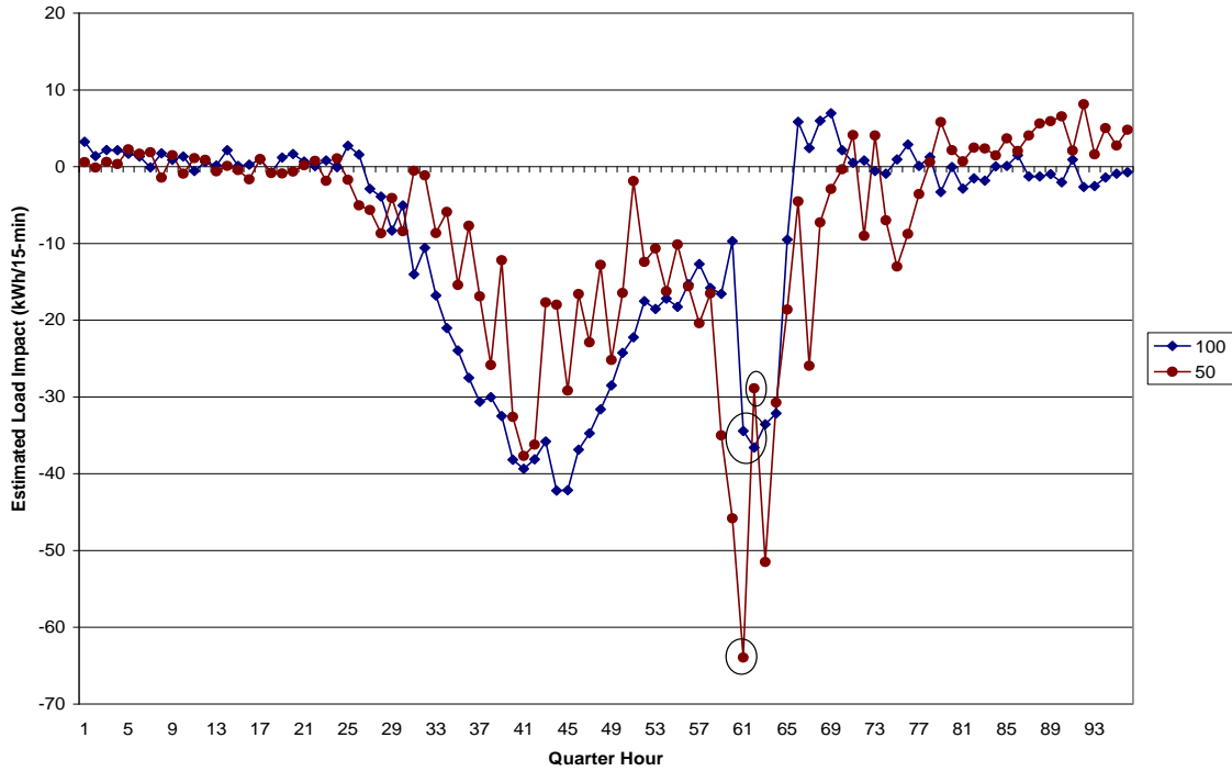
Figure 4-24: Estimated Large Commercial Load Impacts, by Cycling Strategy – September 29 Event (QE 61-64); Villa Park
