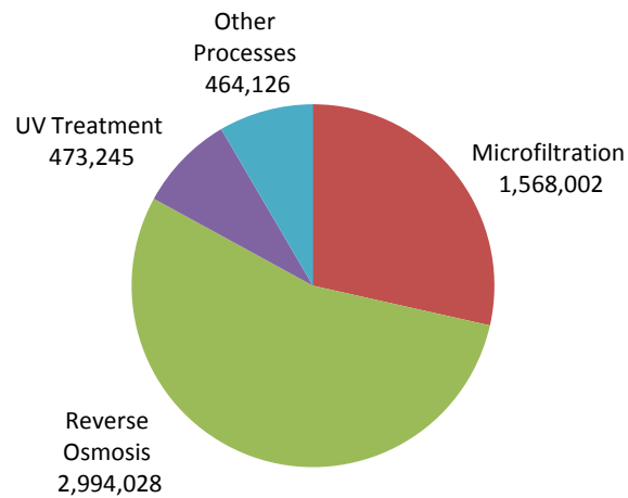
Figure 6: Energy Use by Function (kWh) - December 2008
