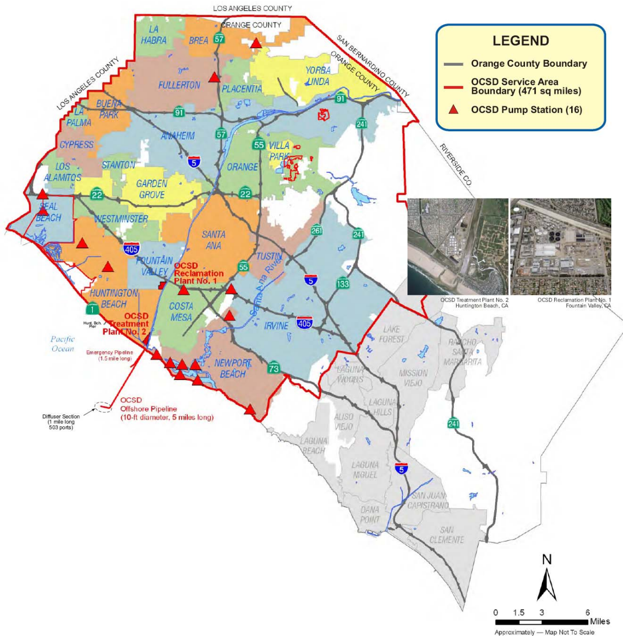
Figure 2: OCWD Infrastructure
