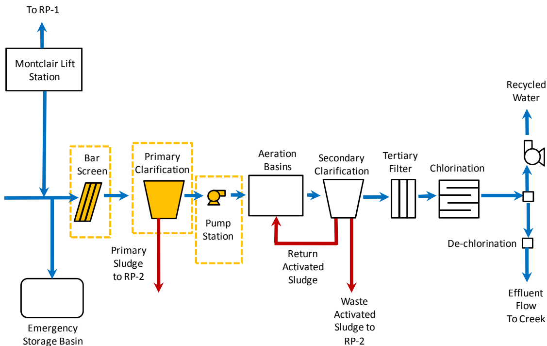
Figure 5: CCWRF Process Flow Diagram
