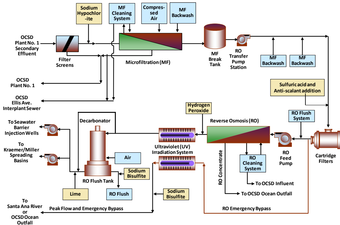
Figure 4: AWP Process Diagram
