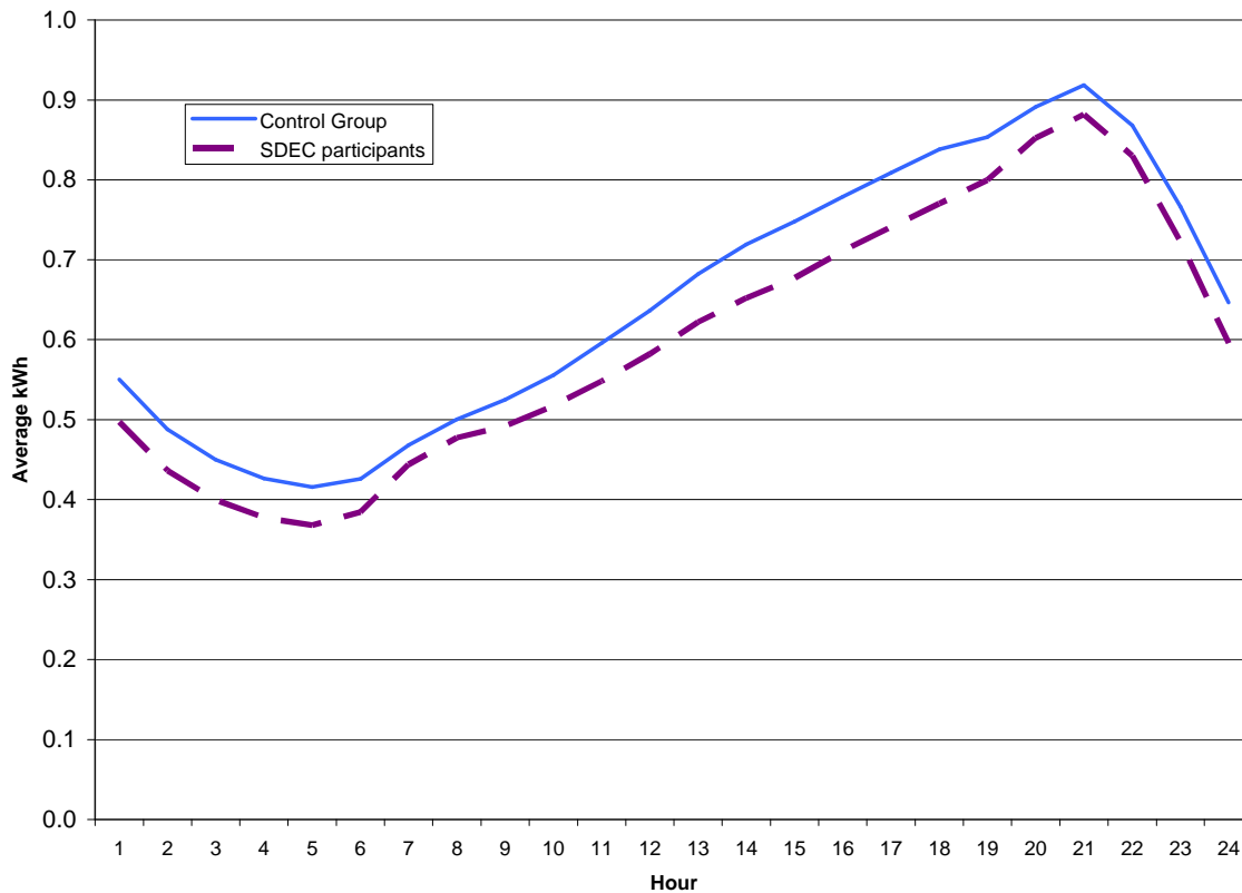
Figure 6–2: Average Daily Load Profiles of SDEC and Control Group Customers – August–September 2012
