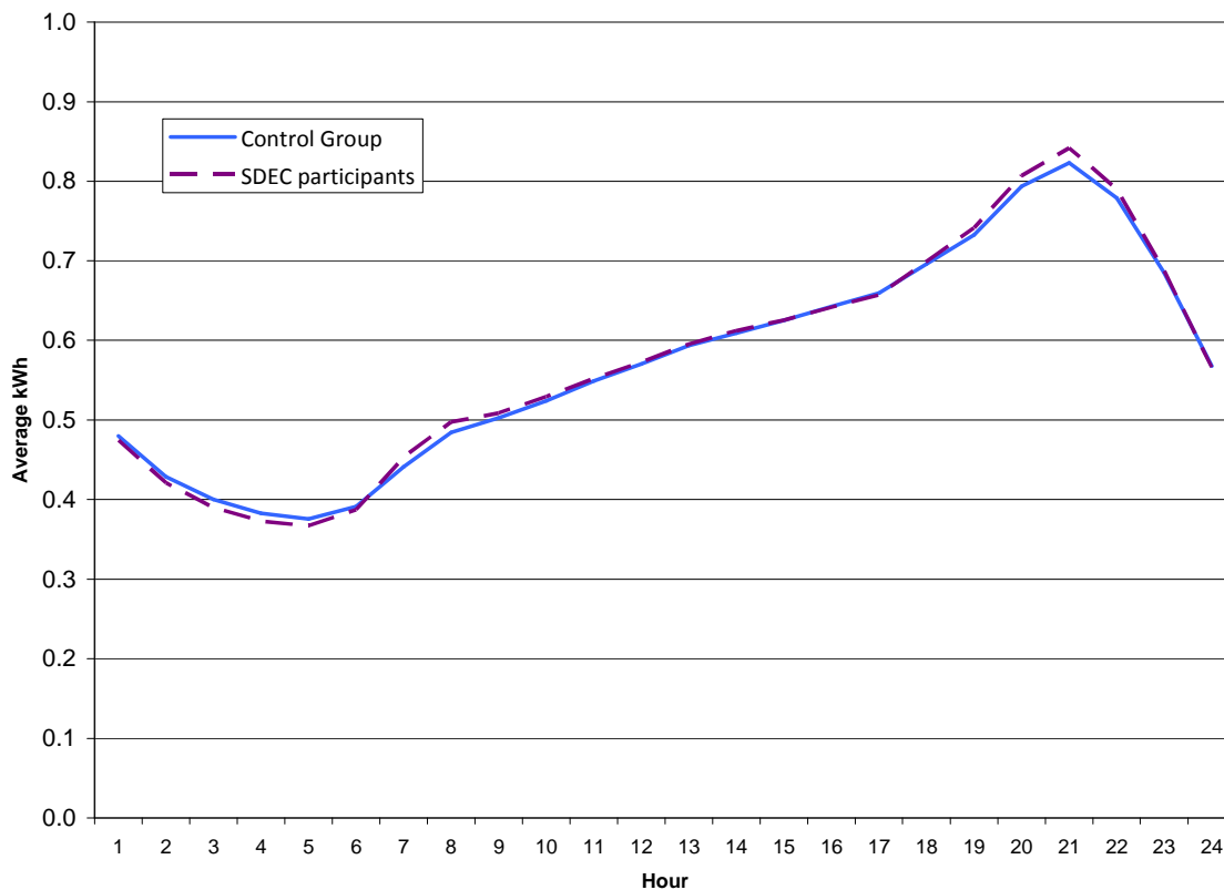
Figure 6–1: Average Daily Load Profiles of SDEC and Control Group Customers – August–September 2011
