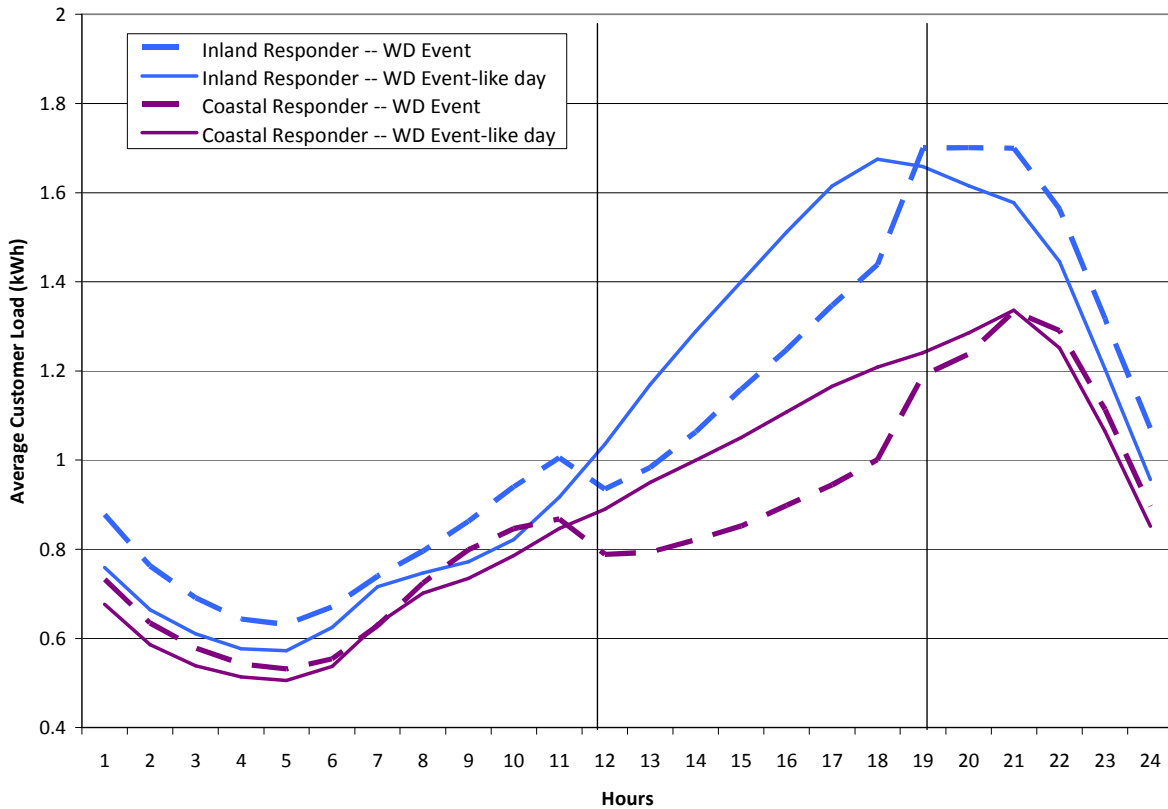
Figure 4–4: Average Load Profiles for Responders on Events and Event-like Days – Opt-in Alert; Coastal and Inland
