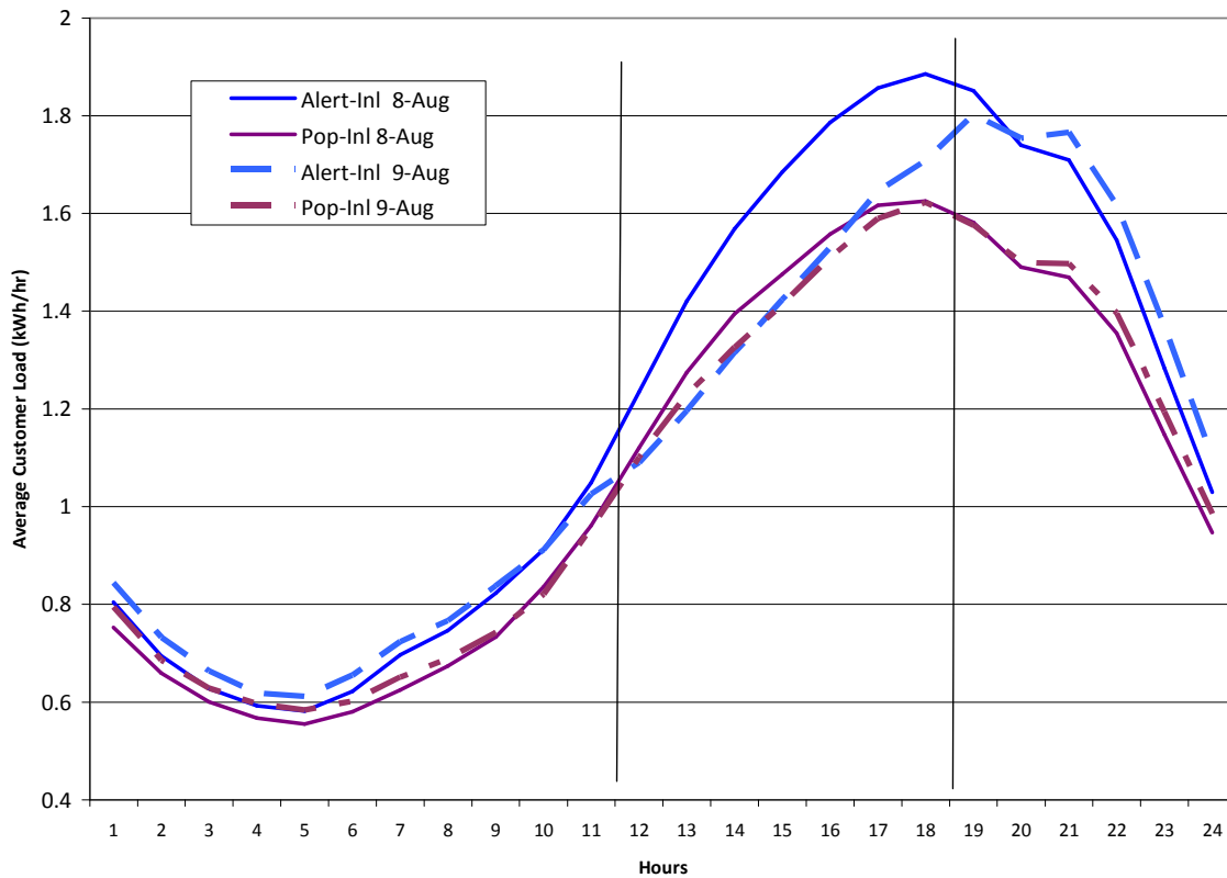
Figure 2–7: Observed Average Customer Loads – August 9 Event Inland; Opt-in Alert and Population
